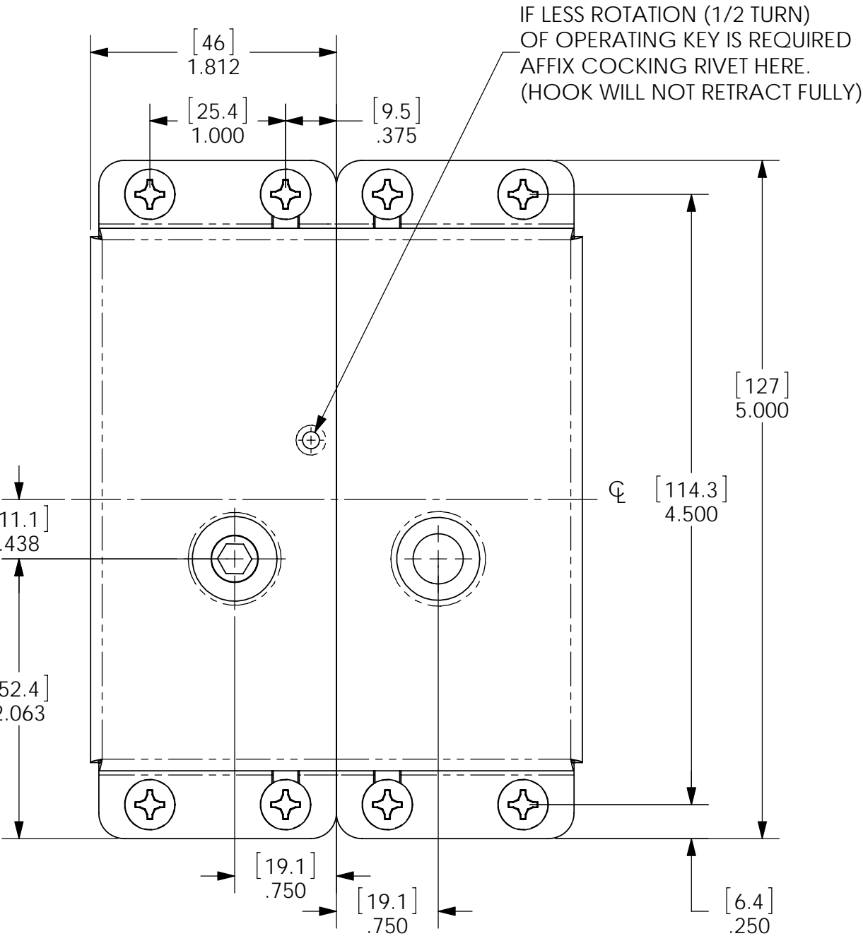
DIMENSIONS WHEN MOUNTED AND LOCKED LATCH AND RECEIVER CASES TOUCH WHEN LOCKED
