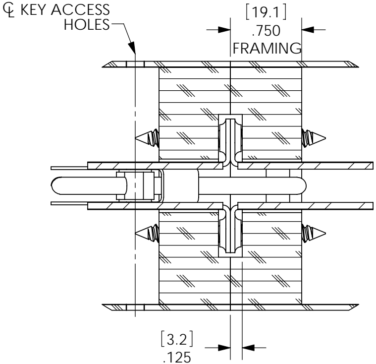
SECTION THRU WALL PANEL
