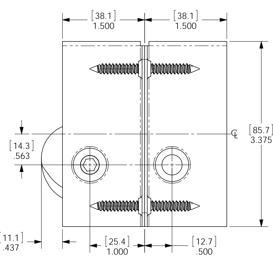
DIMENSIONS WHEN MOUNTED AND LOCKED LATCH AND RECEIVER CASES TOUCH WHEN LOCKED
